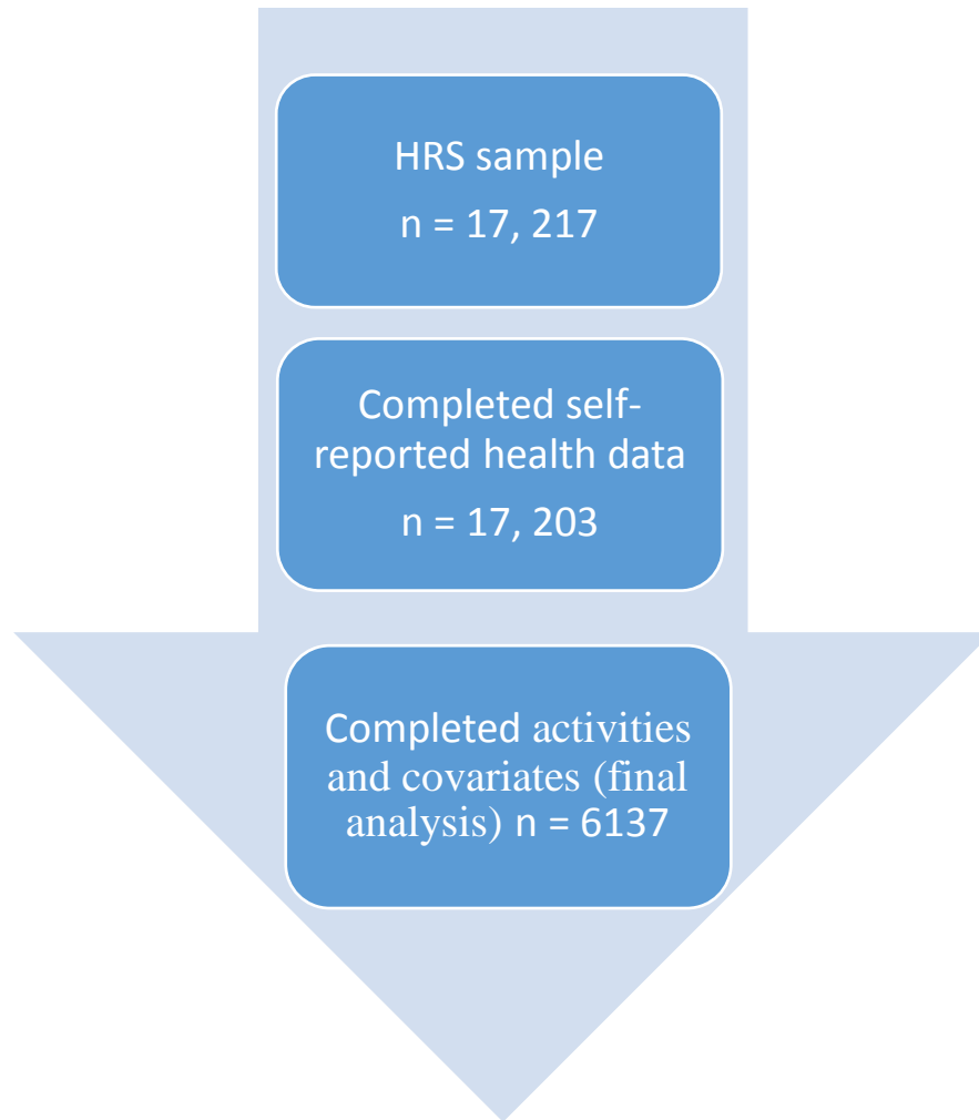
Figure 2. Flow chart and sample for multiple logistic regression analyses.
