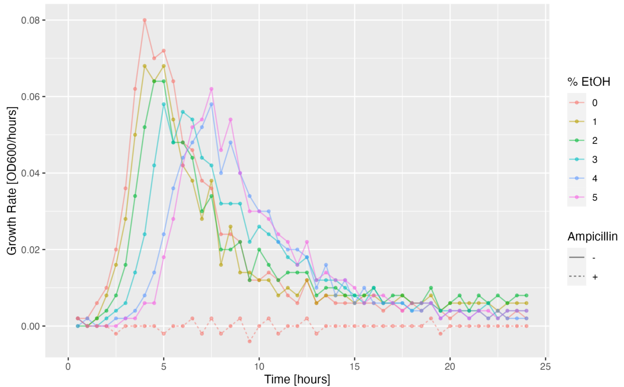
Figure S1: Ethanol decreases the maximum growth rate of BL21(DE3) E. coli .
